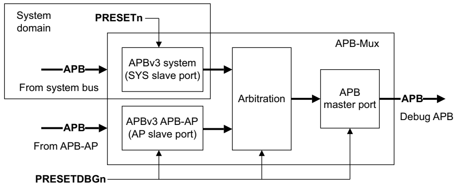
Figure 2-19 APB-Mux domains
